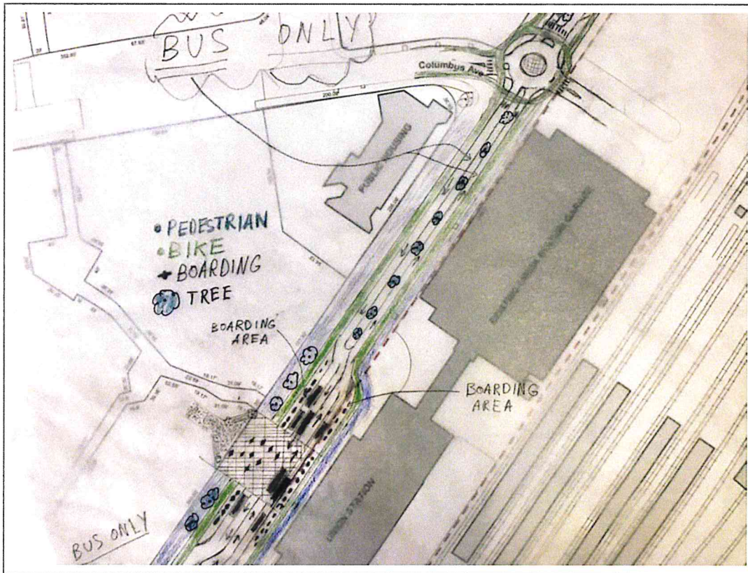
A two-lane shared-street concept showing Union Avenue converted to a transit-only street in the area adjacent to Union Station. Design elements include a landscaped median, bike lanes, enhanced bus boarding areas, a traffic circle at the intersection of Union and Columbus Avenues, and shared-street.
